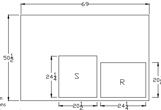
EXISTING UNIT
